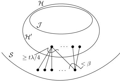
Figure 2. Good \mathcal{S} -vertices have fewer than \beta neighbors in \mathcal{H}' and fewer than \beta^2 neighbors in \mathcal{S} . Good \mathcal{H}' -vertices have at least t\lambda/4 good neighbors in \mathcal{S} .
